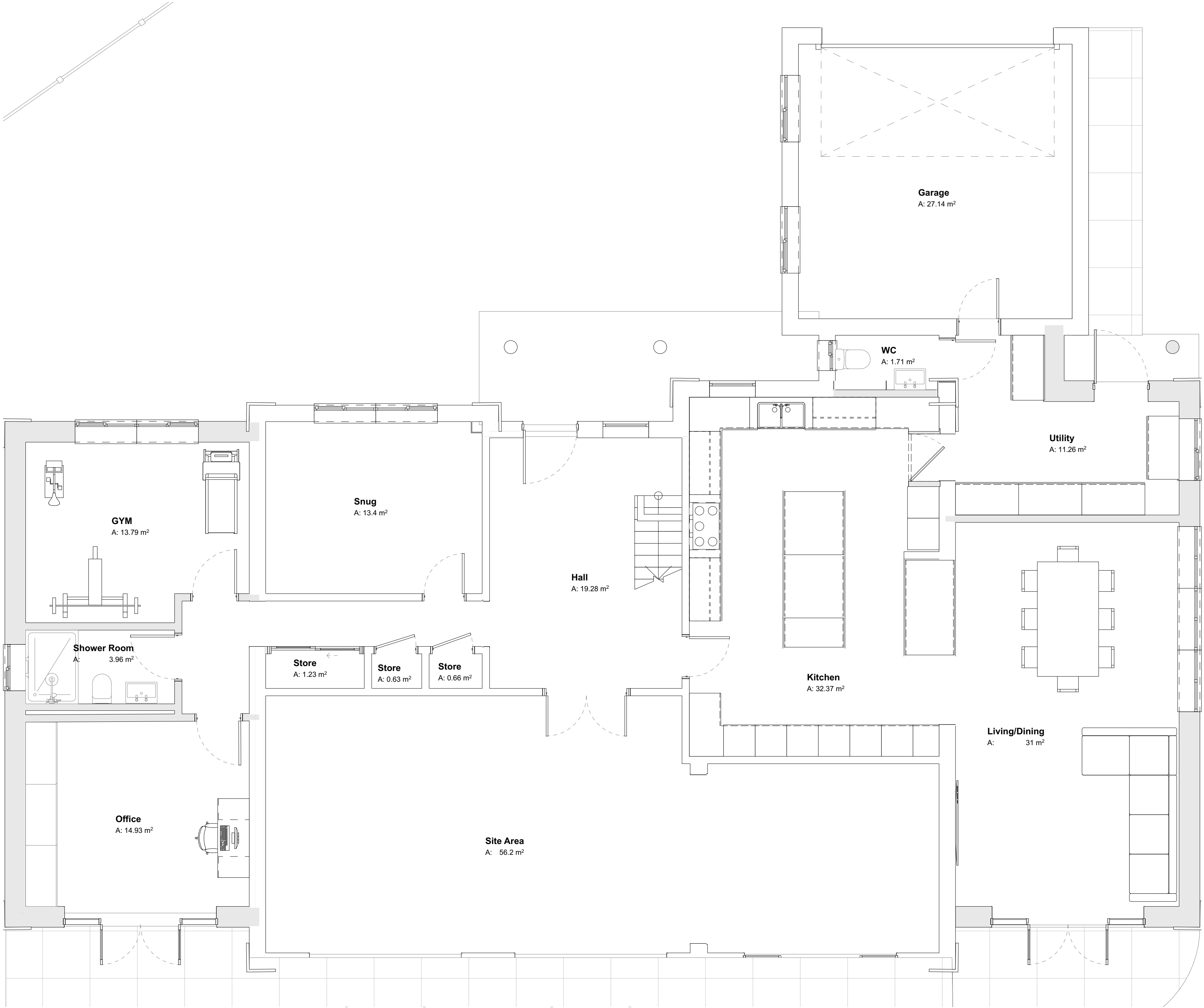
Proposed - Ground Floor GFL 1:50
