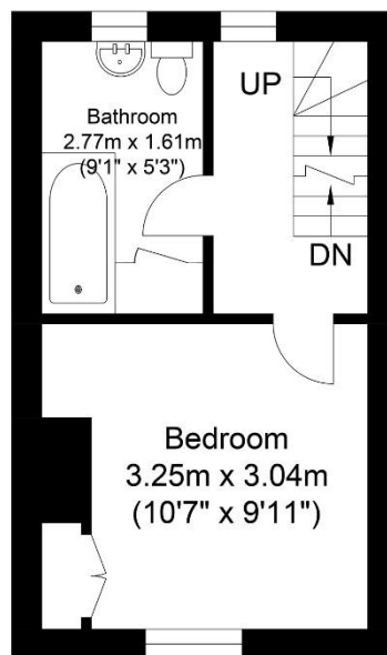
First Floor Approximate Floor Area 204.62 sq ft (19.01 sq m)
