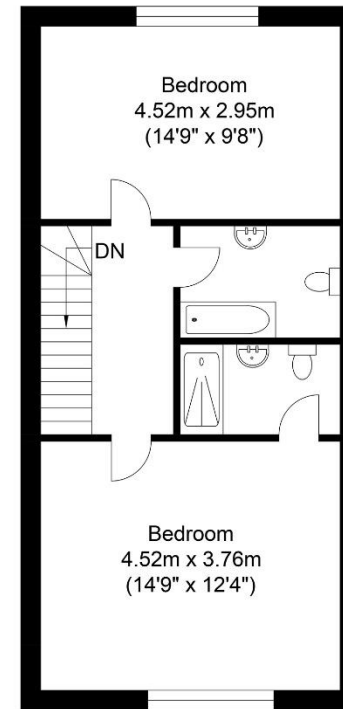
Second Floor Approximate Floor Area 487.60 sq ft (45.30 sq m)
