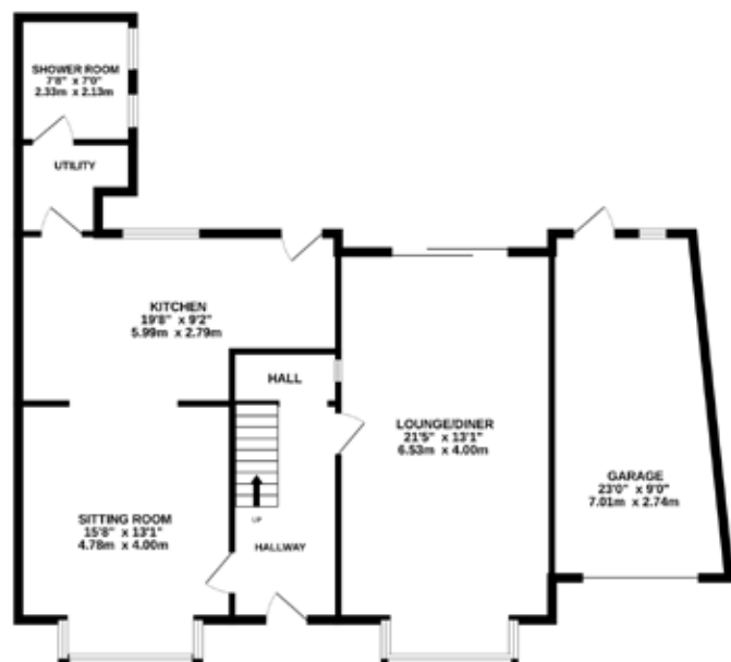
GROUND FLOOR 1092 sq.ft. (101.5 sq.m.) approx.
