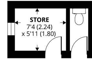
OUTBUILDING 2
