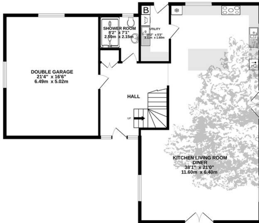
GROUND FLOOR 1292 sq.ft. (120.0 sq.m.) approx.
