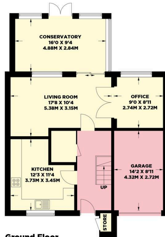
Ground Floor 813 sq Ft / 75.5 sq M
