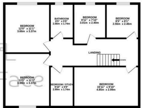
1ST FLOOR 819 sq.ft. (76.1 sq.m.) approx.
