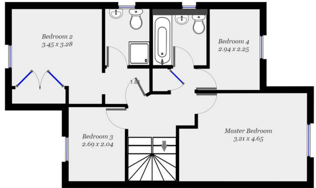
FIRST FLOOR - 64.90 Sq. M (700 Sq. Ft)
