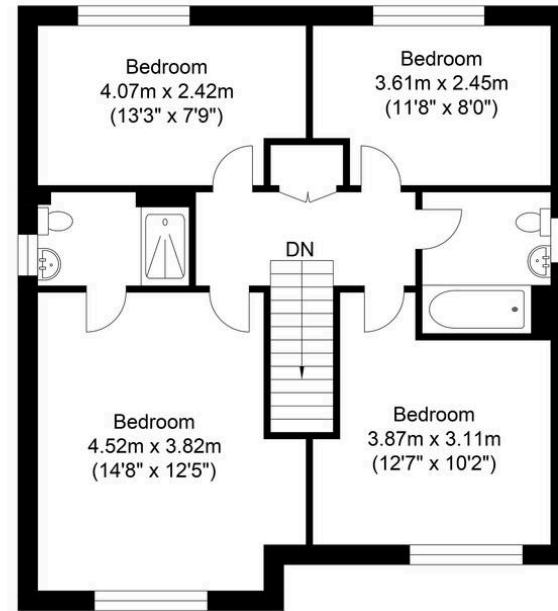
First Floor Approximate Floor Area 684.15 sq ft (63.56 sq m)
