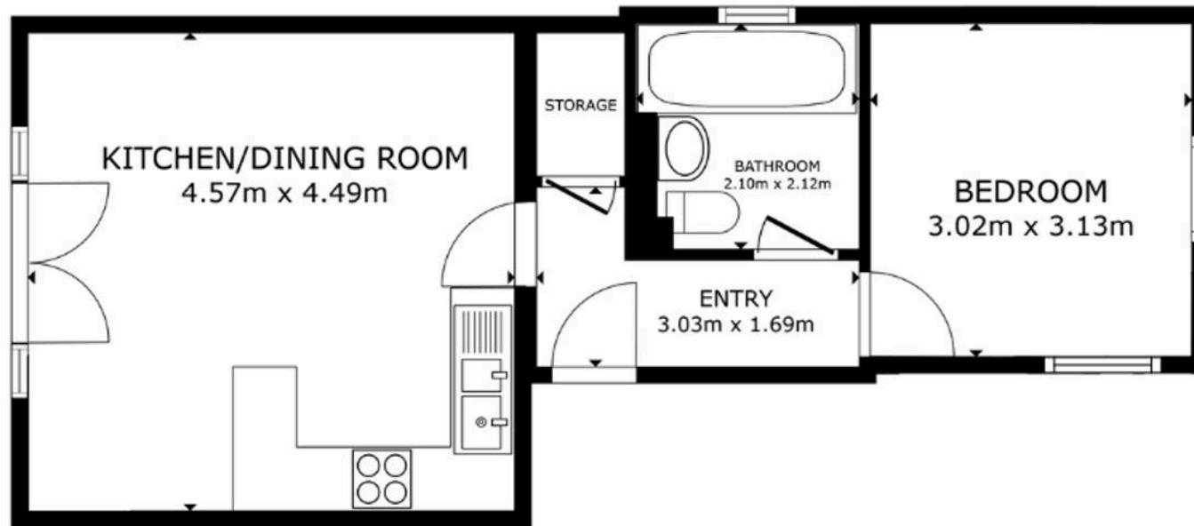
FLOOR PLAN
