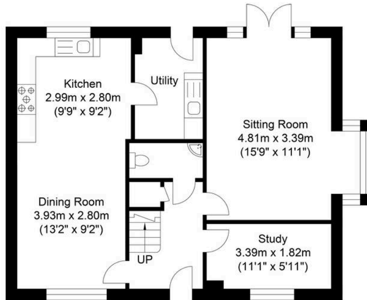
Ground Floor Approximate Floor Area 624.62 sq ft (58.03 sq m)
