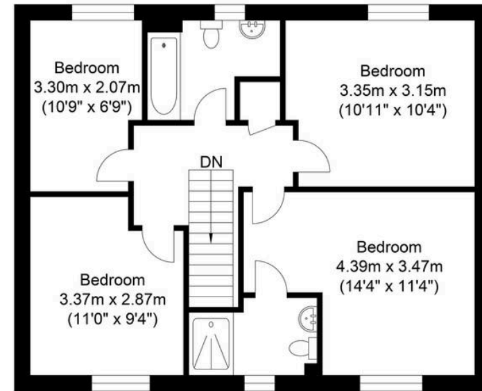
First Floor Approximate Floor Area 610.52 sq ft (56.72 sq m)
