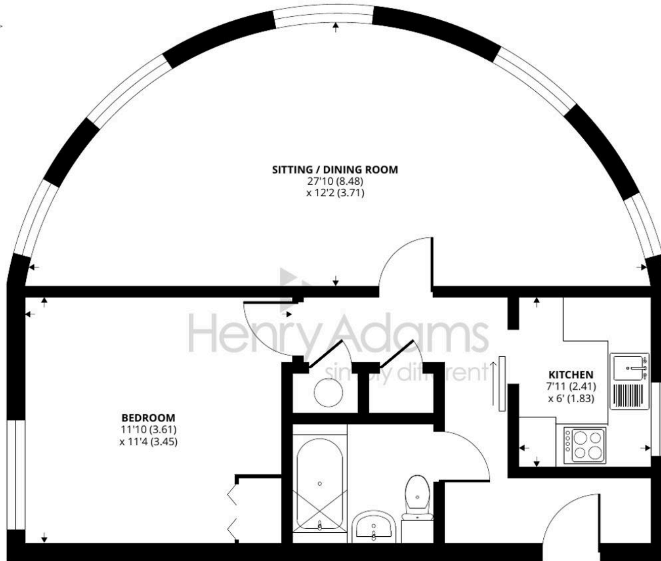
FIRST FLOOR
