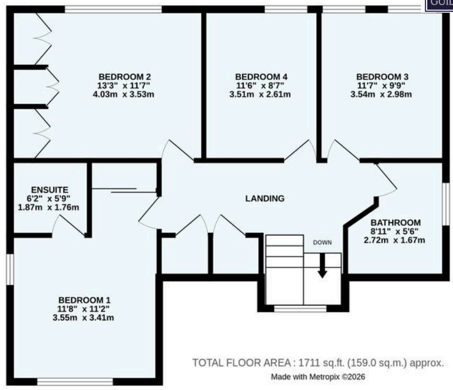
1ST FLOOR 829 sq.ft. (77.0 sq.m.) approx.
