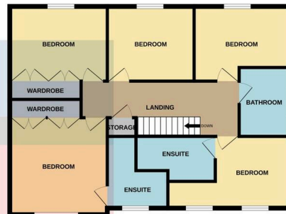
1ST FLOOR 862 sq.ft. (80.1 sq.m.) approx.
