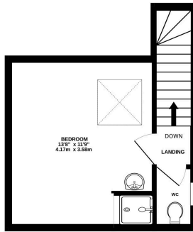
1ST FLOOR 219 sq.ft. (20.4 sq.m.) approx.
