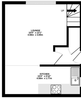
GROUND FLOOR 270 sq.ft. (25.0 sq.m.) approx.
