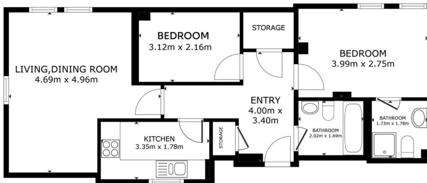
FLOOR PLAN
