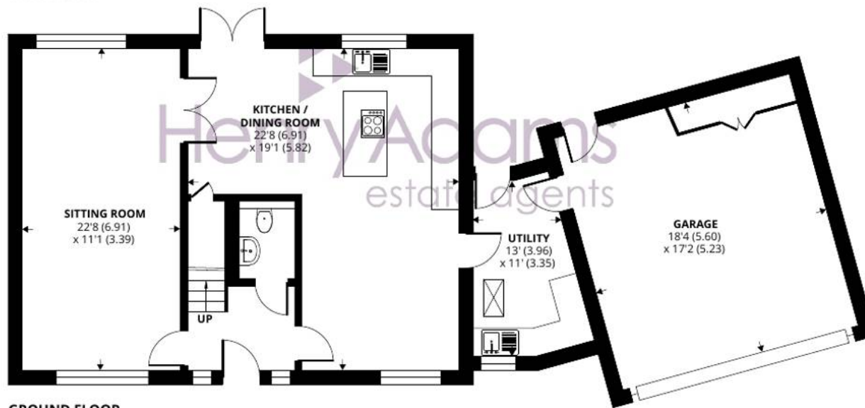
GROUND FLOOR
