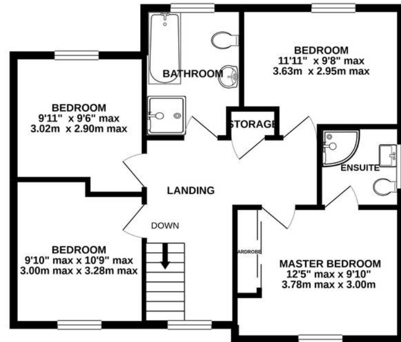
1ST FLOOR 663 sq.ft. (61.6 sq.m.) approx.
